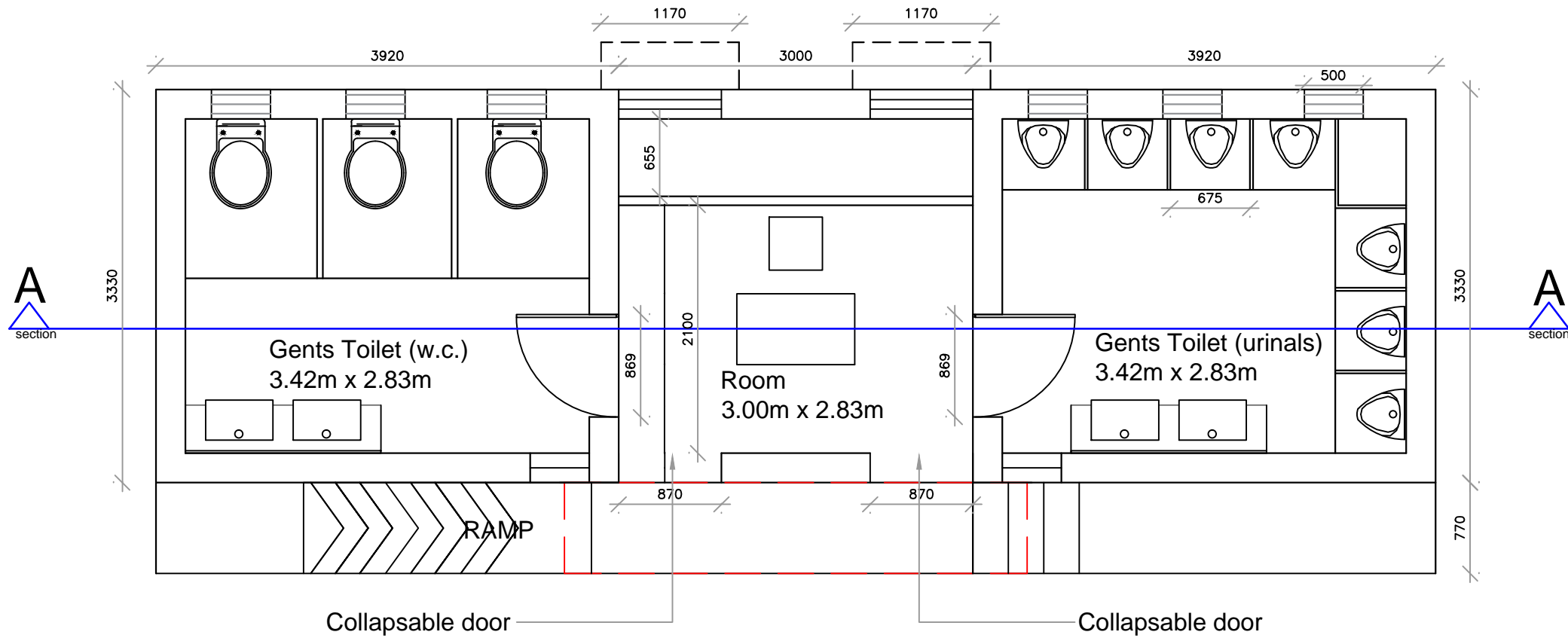
NEW MODIFIED GENT'S TOILET LAYOUT
